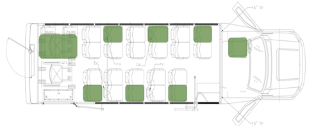
Grech Ford E-550 ADA with typical 24 passengers seat layout following CDC guidelines of 6' of social distancing
