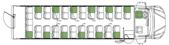
Grech with typical 48 passengers seat layout following CDC guidelines of 6' of social distancing
