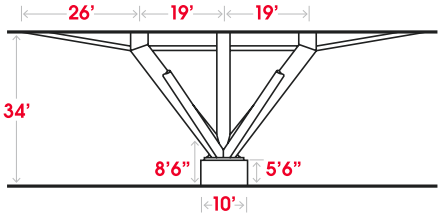
COLUMN POSITION FACING SIDES OF BUILDING
