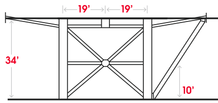
COLUMN POSITION FACING SIDES OF BUILDING HALLS A, B, D, E ONLY
