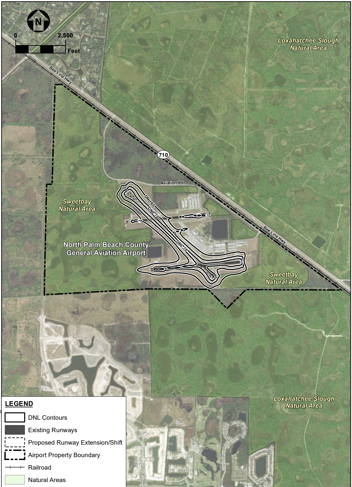
North Palm Beach County General Aviation Airport Runway Extension FIGURE B-9 PROPOSED PROJECT: 2025 DNL CONTOURS AT F45
