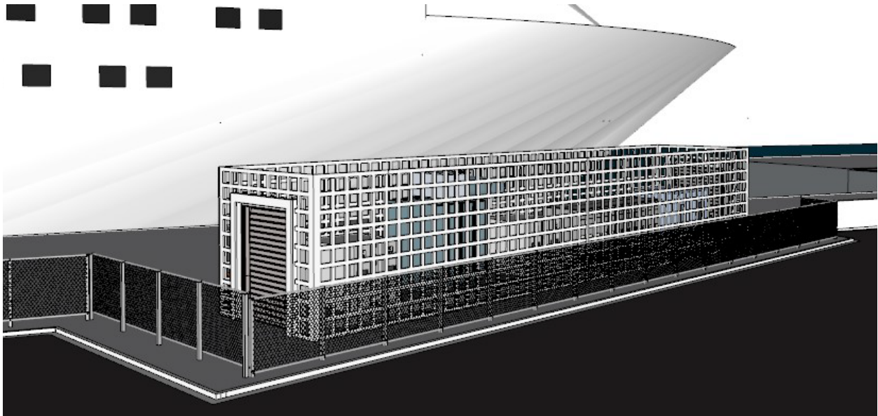
Figure 4-4. Concept 4: Traditional Equipment Line-up, Single Vessel (Architectural Shrouding)
