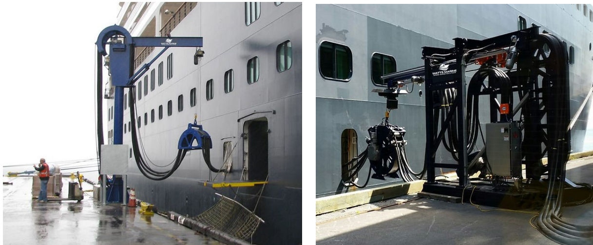
Figure 2-6. Fixed and Repositionable Jib Crane Examples
