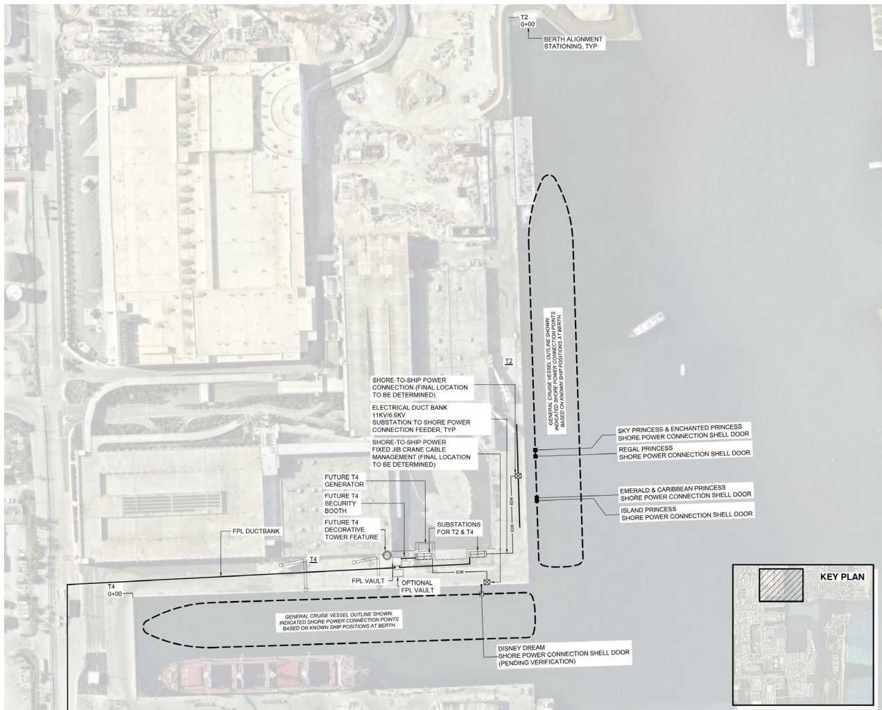
Figure 5-2. CT2 and CT4 Enlarged Electrical Site Plan (Sheet E111)
