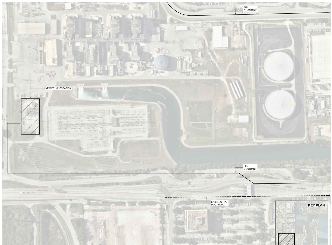
Figure 5-6. Enlarged Electrical Site Plan for FPL New Substation (Sheet E115)
