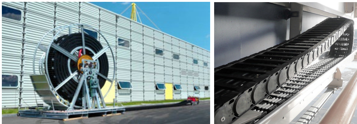
Figure 2-8. Cable Reel and Chain Enclosure Examples
