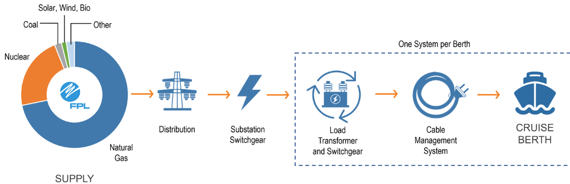
Figure 1-1. Primary Components of Shore Power with FPL as Energy Provider
