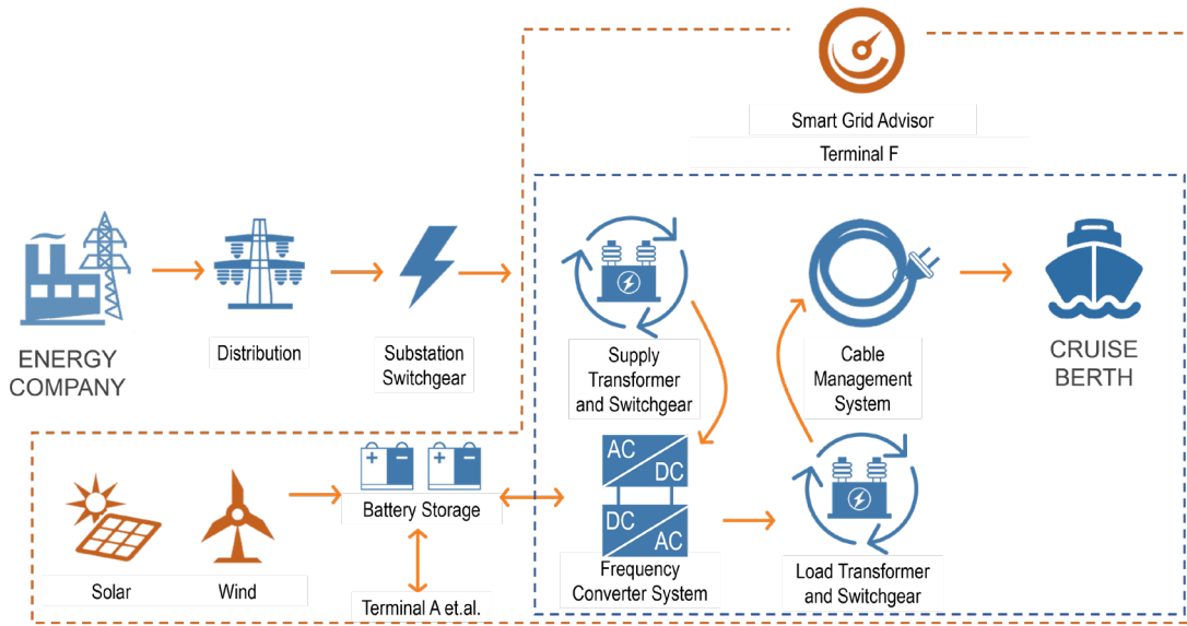
Figure 10-1. Shore Power Supply with Power Factor Conversion Linked to Microgrid
