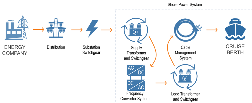
Figure 2-2. Traditional Shore Power System with Power Factor Conversion
