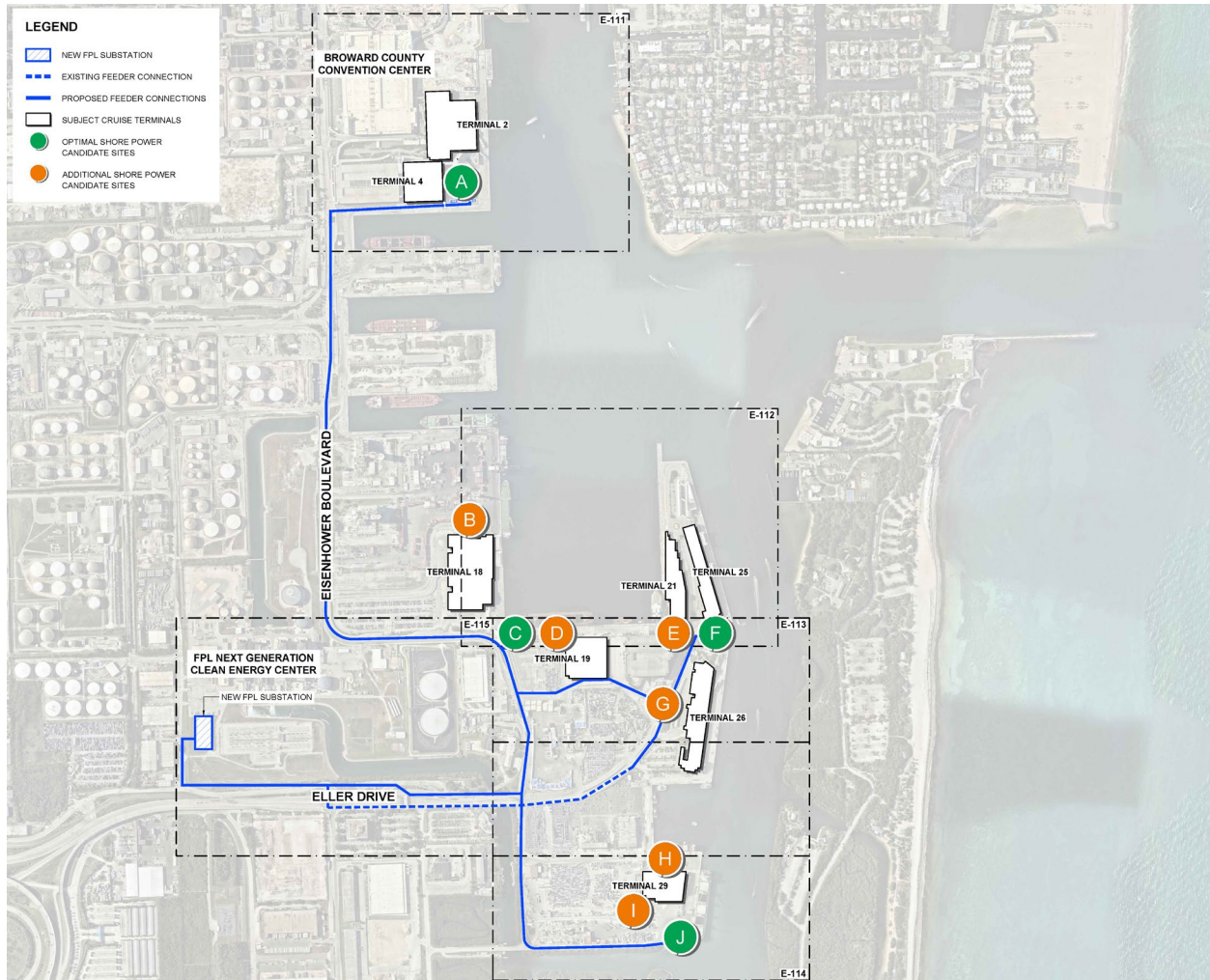
Figure 4-7. Cruise Terminal F Shore Power Candidate Sites
