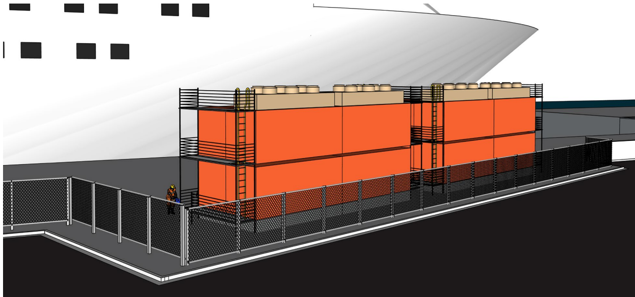
Figure 4-6. Concept 6: Containerized, Two Vessels (Architectural Shrouding)
