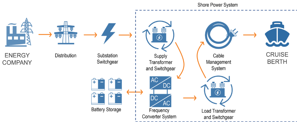
Figure 2-3. Conventional Shore Power with Modular Grid Energy Storage
